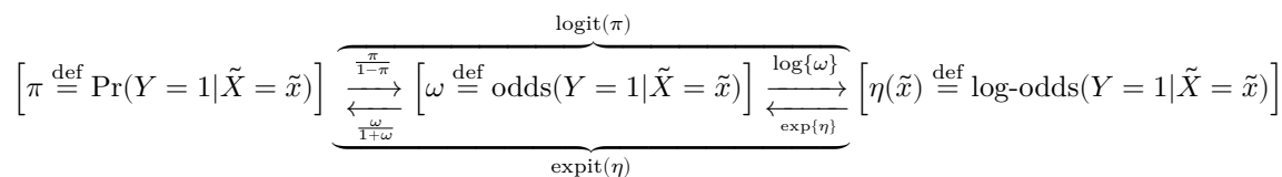
Figure 6: Diagram of logistic regression link and inverse link functions
