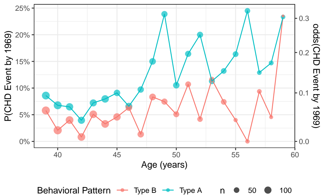
Figure 12: CHD rates by age group, probability scale
