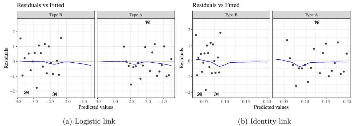
Figure 21: Residuals vs Fitted plot for wcfgs models
