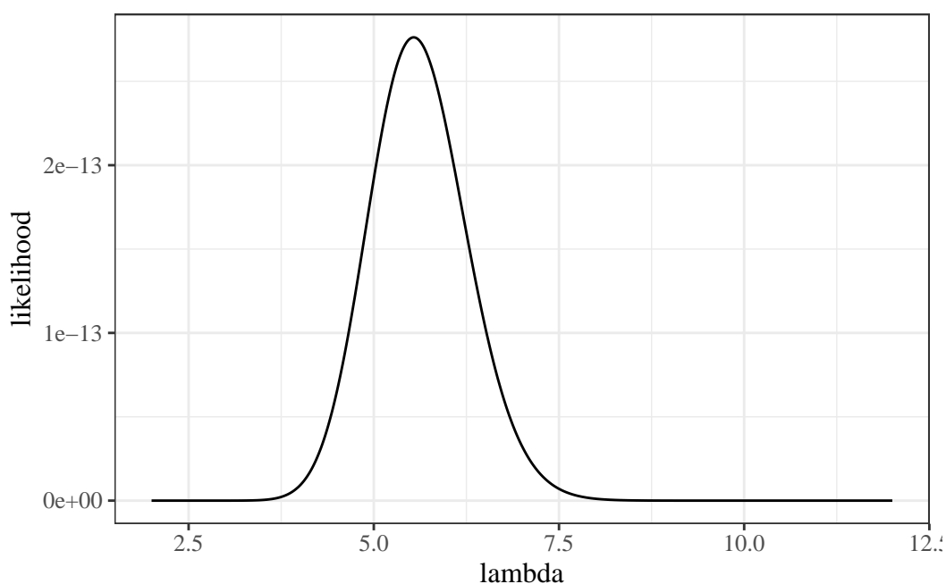
Figure F.3.: Likelihood of Dobson cyclone data
