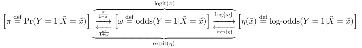
Figure 3.6.: Diagram of logistic regression link and inverse link functions
