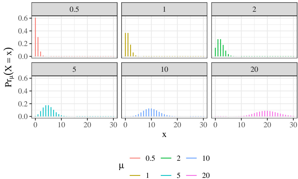
Figure C.2.: Poisson PMFs, by mean parameter \mu
