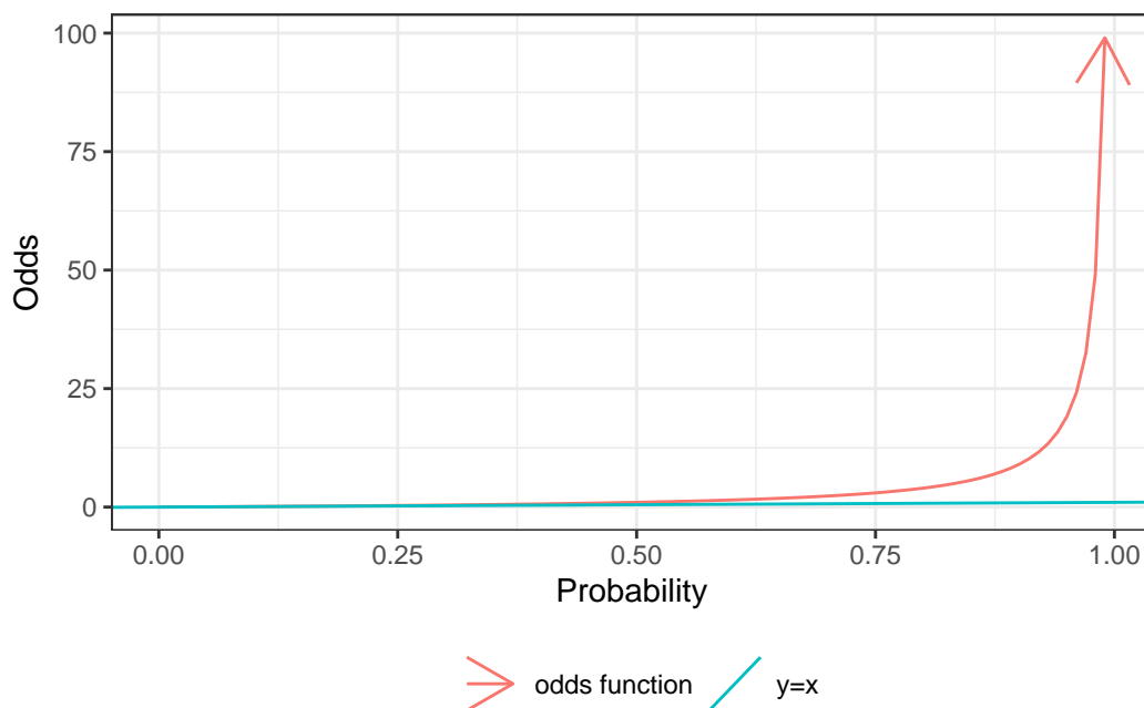
Figure 3.1.: Odds versus probability
