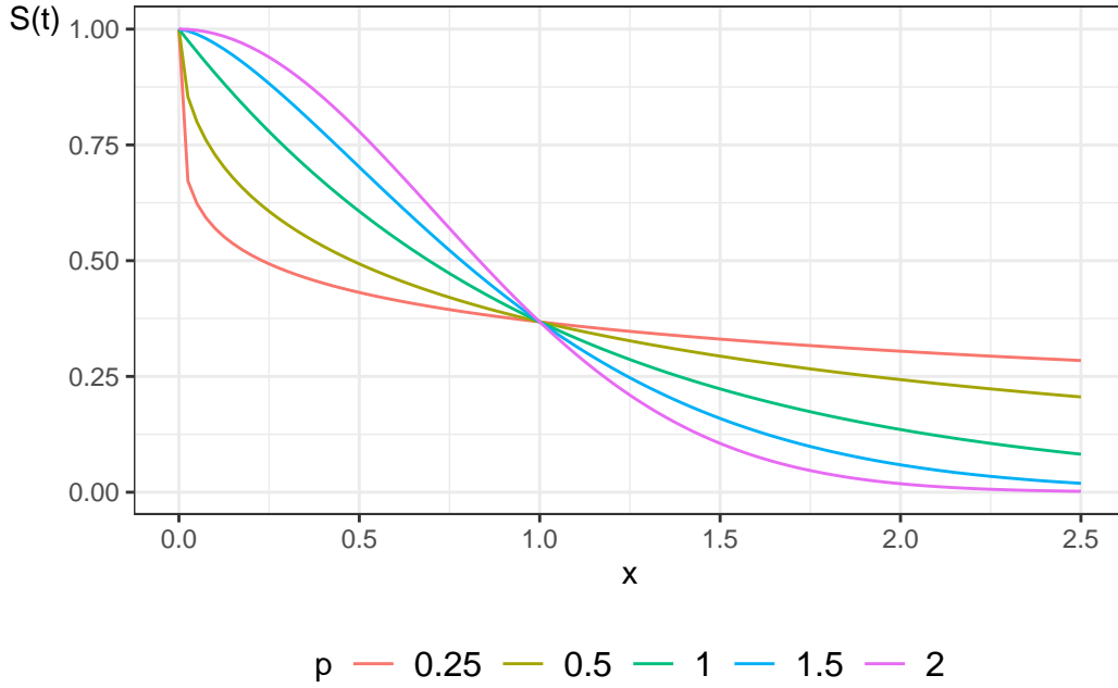
Figure 8.3.: Survival functions for Weibull distribution
