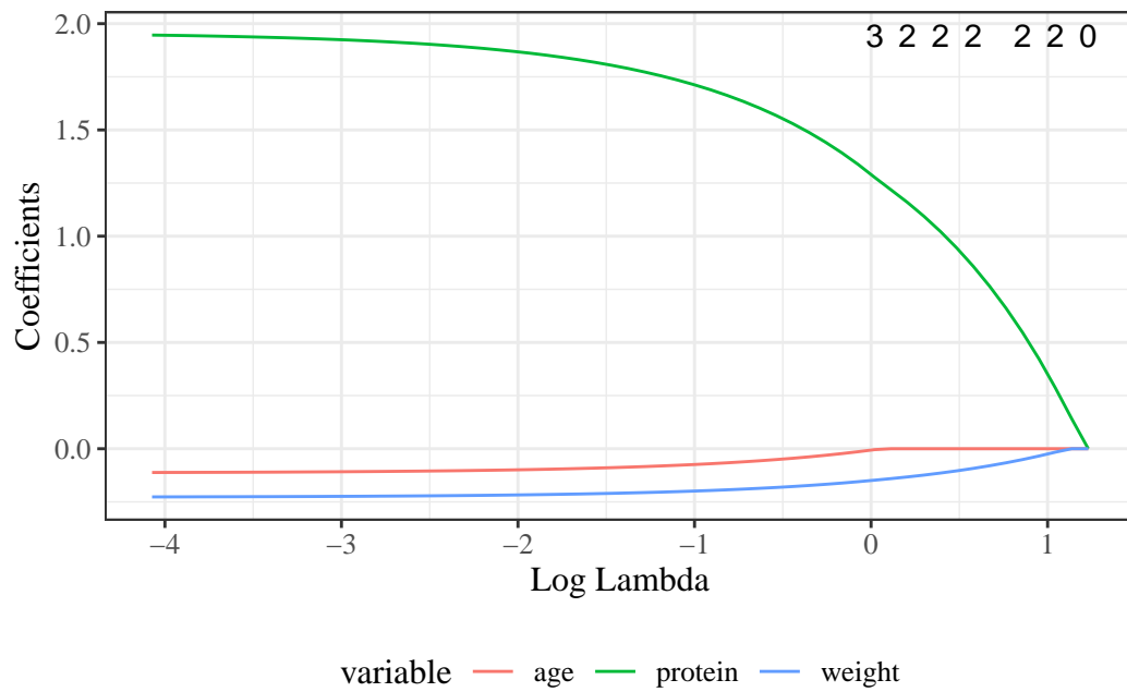
Figure 2.31.: Lasso selection
