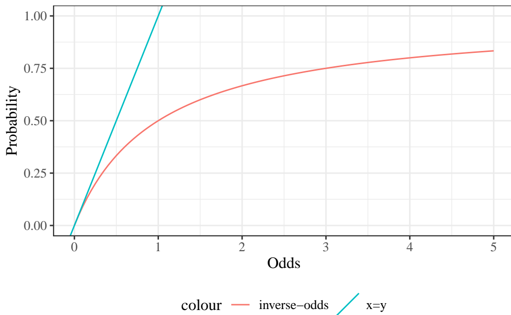
Figure 3.2.: The inverse odds function, \text{invodds}\{\omega\}
