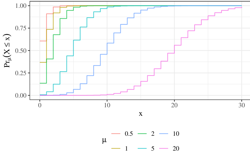
Figure C.3.: Poisson CDFs
