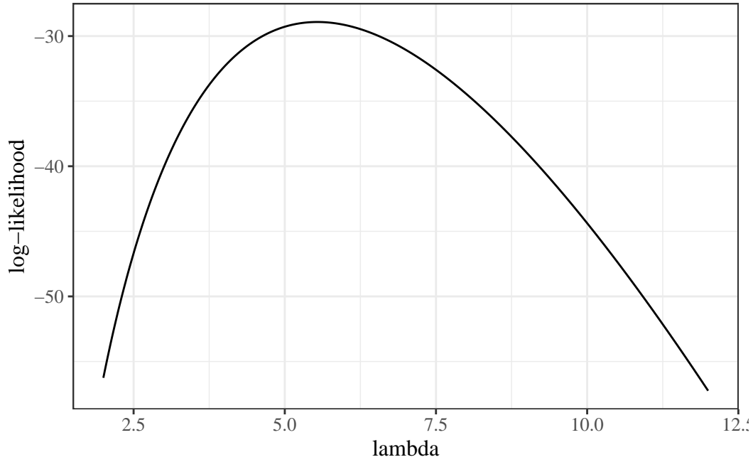
Figure F.4.: log-likelihood of Dobson cyclone data
