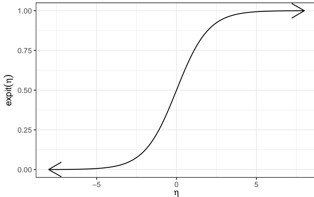
Figure 3.5.: The expit function
