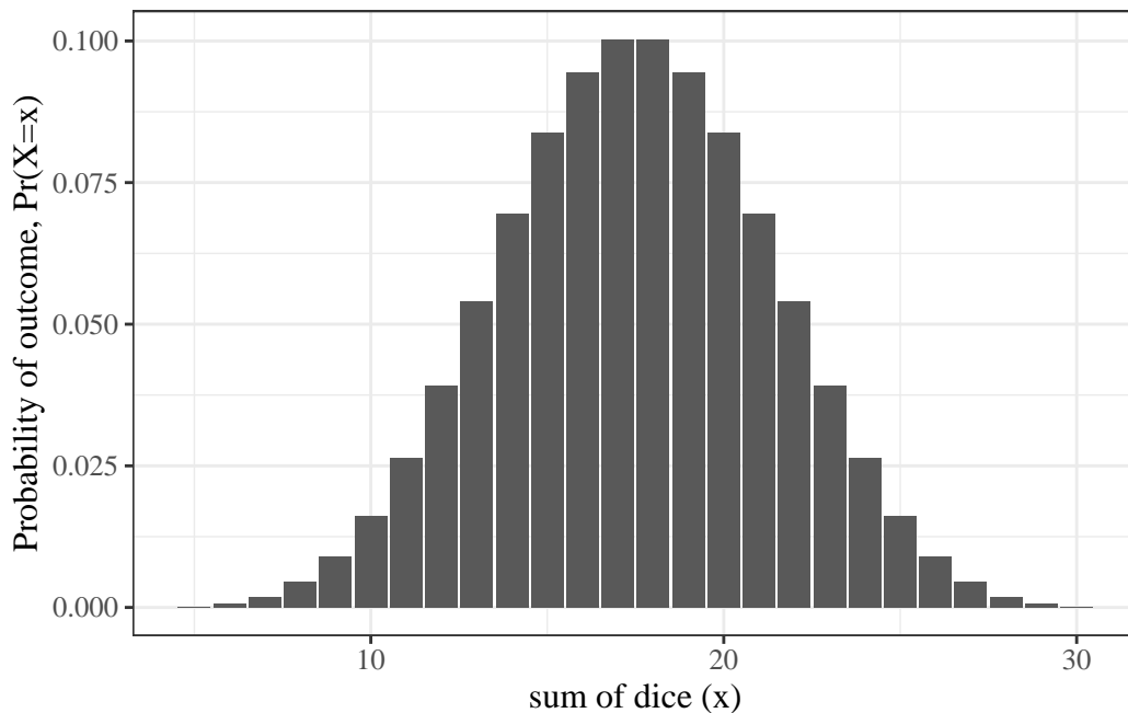
Figure C.4.: Distribution of the sum of five dice
