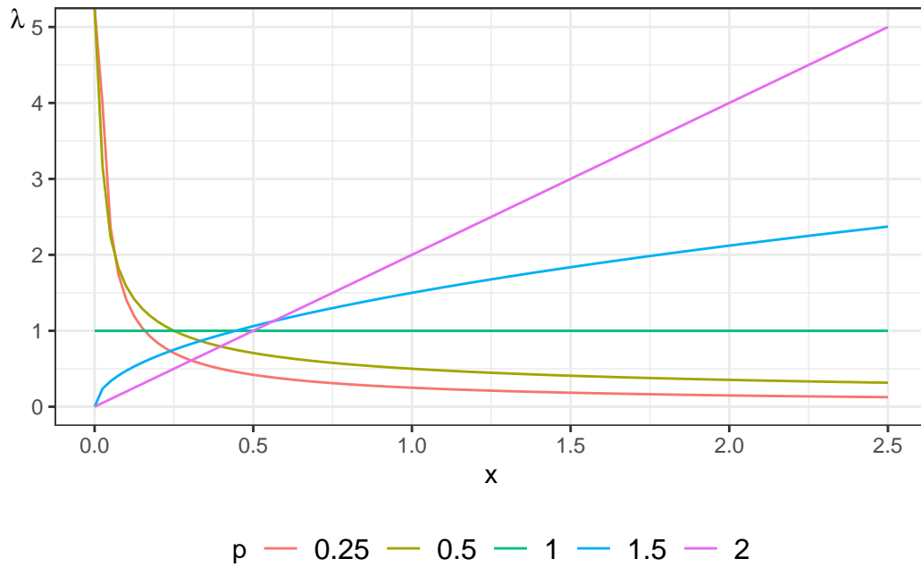
Figure 8.2.: Hazard functions for Weibull distribution
