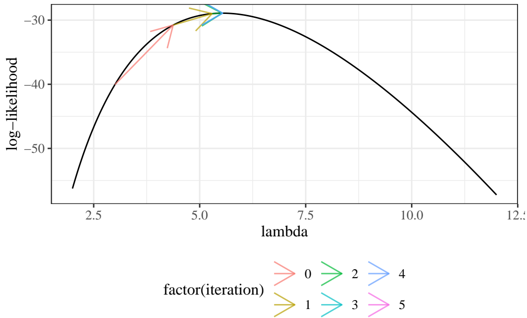
Figure F.13.: Newton-Raphson algorithm for finding MLE of model F.13 for cyclone data
