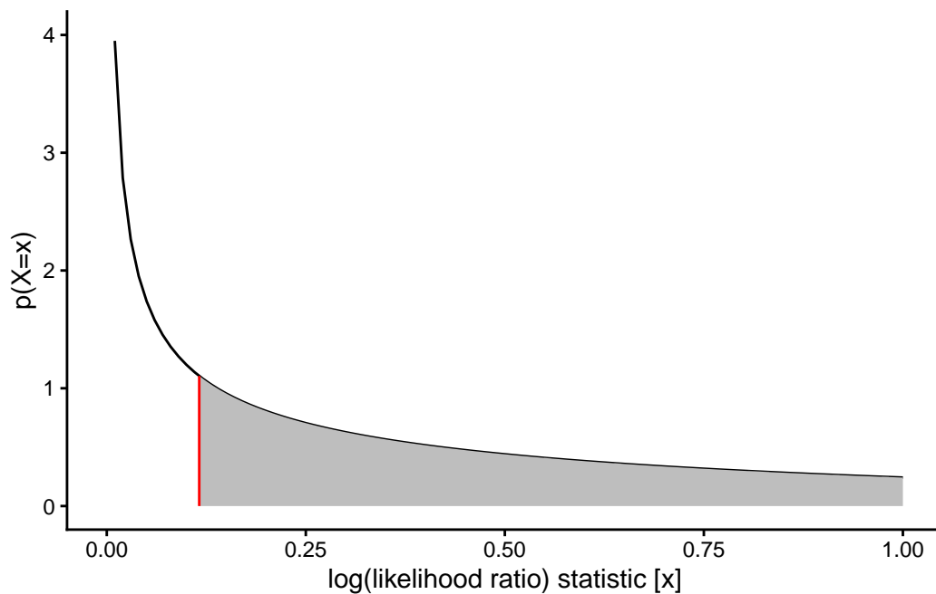
Figure 2.6.: Chi-square distribution
