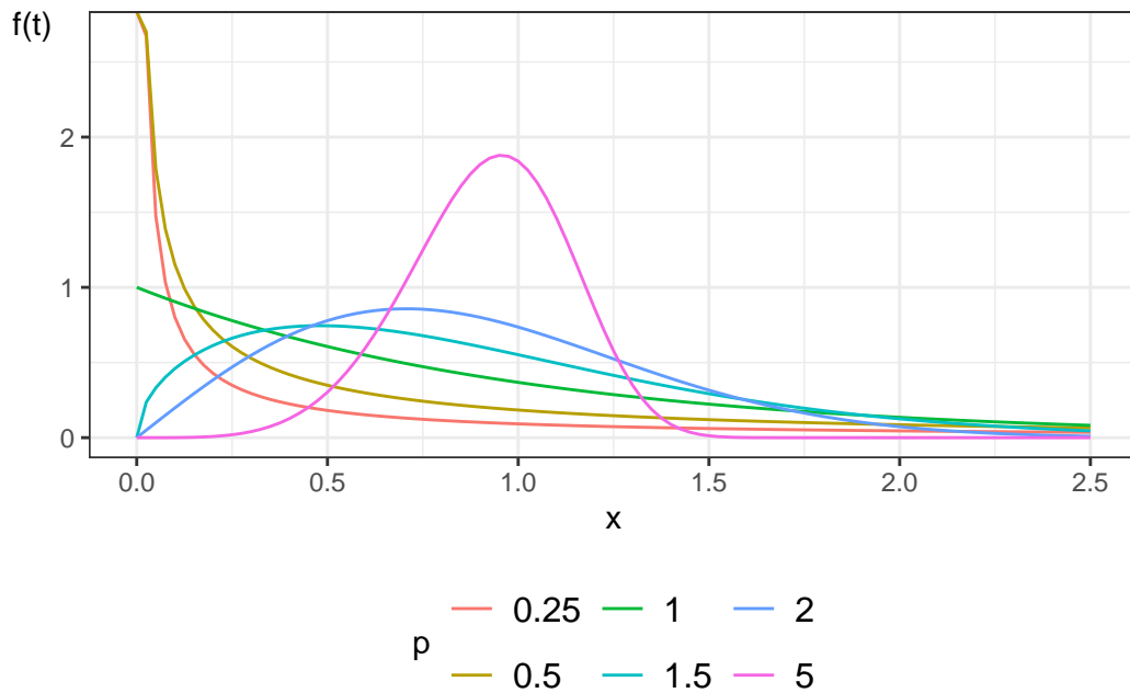
Figure 8.1.: Density functions for Weibull distribution
