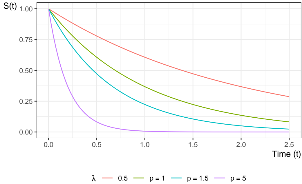
Figure 6.1.: Exponential Survival Functions
